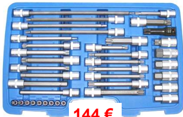
BGS5184 38-delig set - Jeu 38 pièces 1/4 TS10-TS20 / 1/2 RIBE 7x240-8x240 9x100-10x140 / 1/2 TX40-->TX70x140 1/2 IN7-10-11-13x140 + 14-->24 x55mm XZN 9x100+10-12-14x140+16x55-16x100 XZN 18 - TX80x100 - TTX30x300-INB5x160
